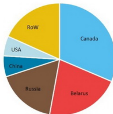
Potash Reserves Globally (K 2 O equivalent)
