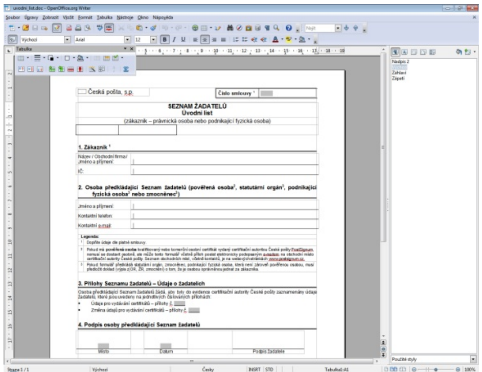
OpenOffice.org Writer
